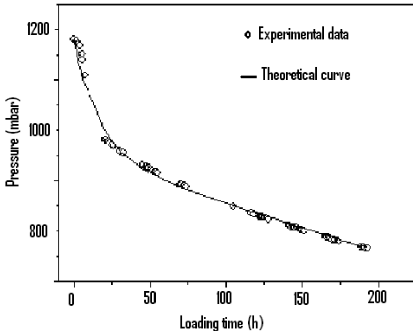
Fig. 4 - Pressure trend as a function of time
