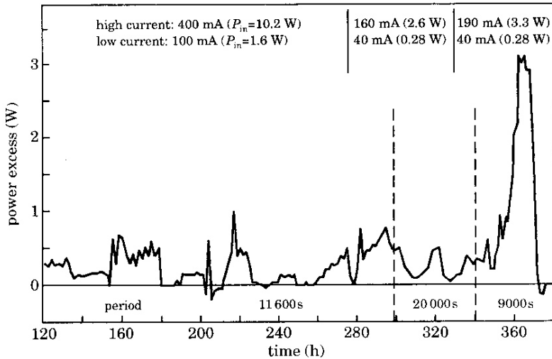
Fig. 5 – Graph of power excess as a function of time, obtained in the second run of the experiment performed in 1992
